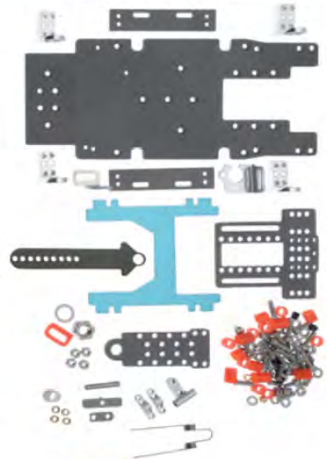
SC-8000b Complete chassis kit Pre-2012
